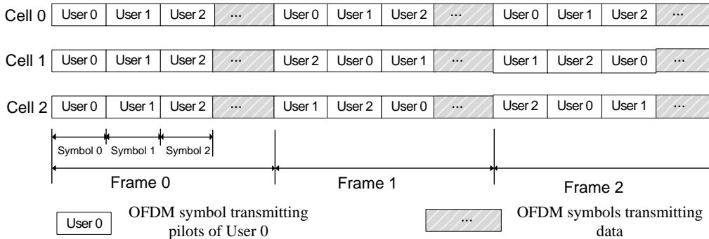
Fig. 2. Illustration of the proposed pilot assignment.
