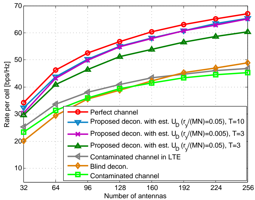
Fig. 6. Achievable sum rate per-cell vs. the number of antennas M .
