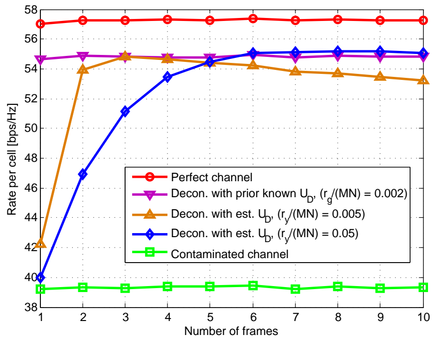
Fig. 5. Achievable sum rate per-cell vs. the number of frames T , M = 128 .
