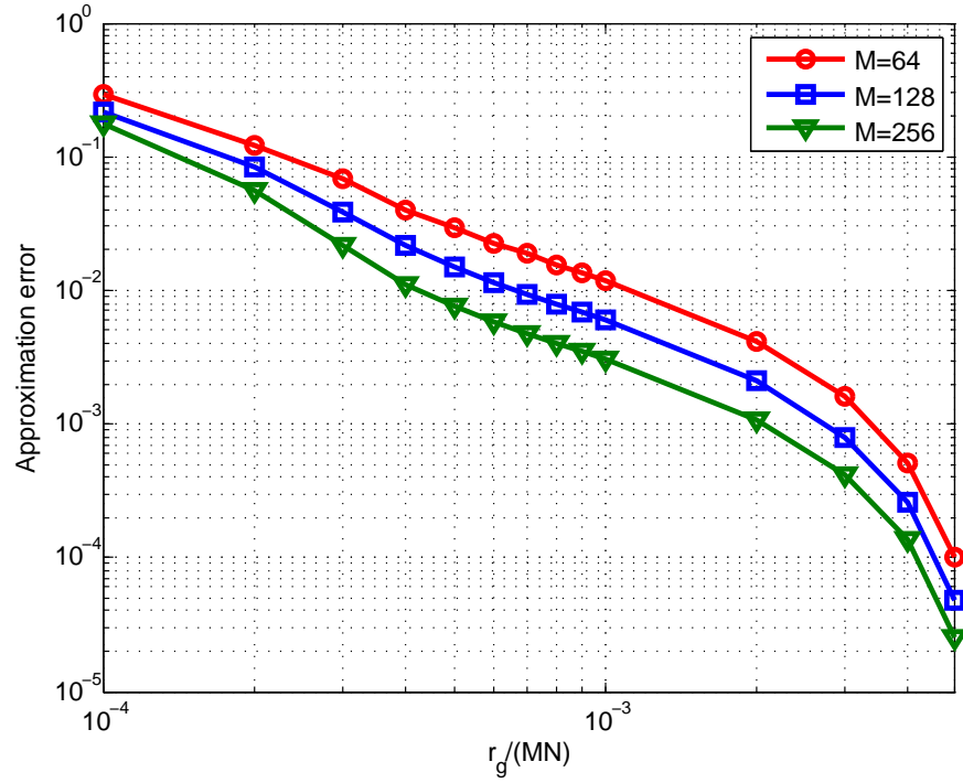
Fig. 3. Approximation accuracy of the DFT representation in (13).
