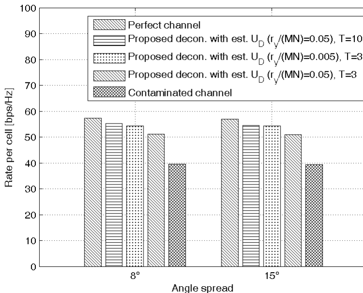
Fig. 7. Achievable sum rate per-cell vs. the angle spread, M = 128 .
