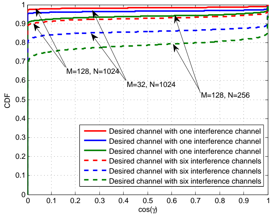
Fig. 4. CDF of the principle angles between the subspaces of the desired channel and the interference channel(s).
